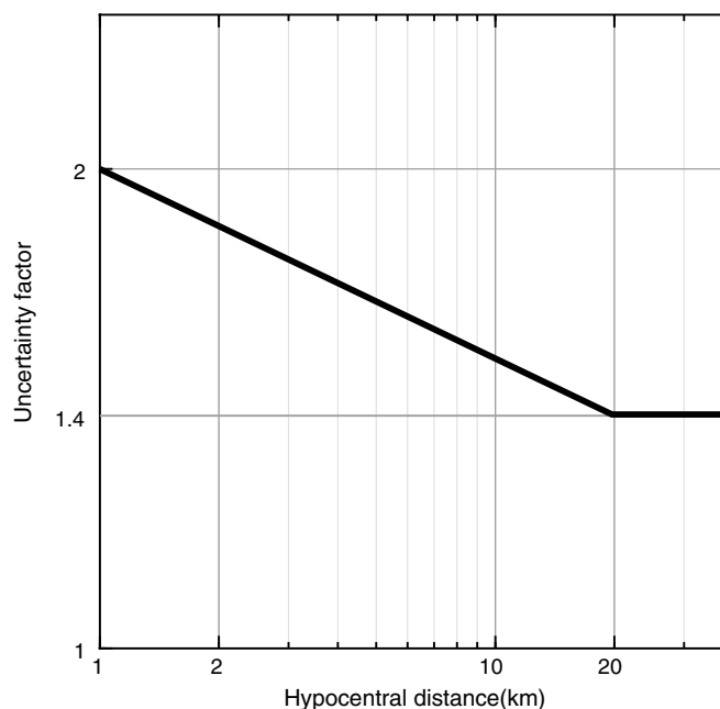
▲ Figure 4. Epistemic uncertainty model for the GMPE as a function of distance relative to the central model. This factor multiplies the central A15 GMPE variant with the Yenier and Atkinson (2014) saturation term and divides the central A15 GMPE variant with the alternative saturation term.
